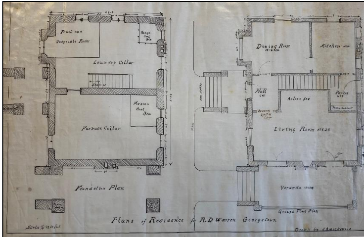
Figure 7: Architectural floorplan drawings for 2 Guelph Street (EHS ARCHIVES MG12 C6 #15)
