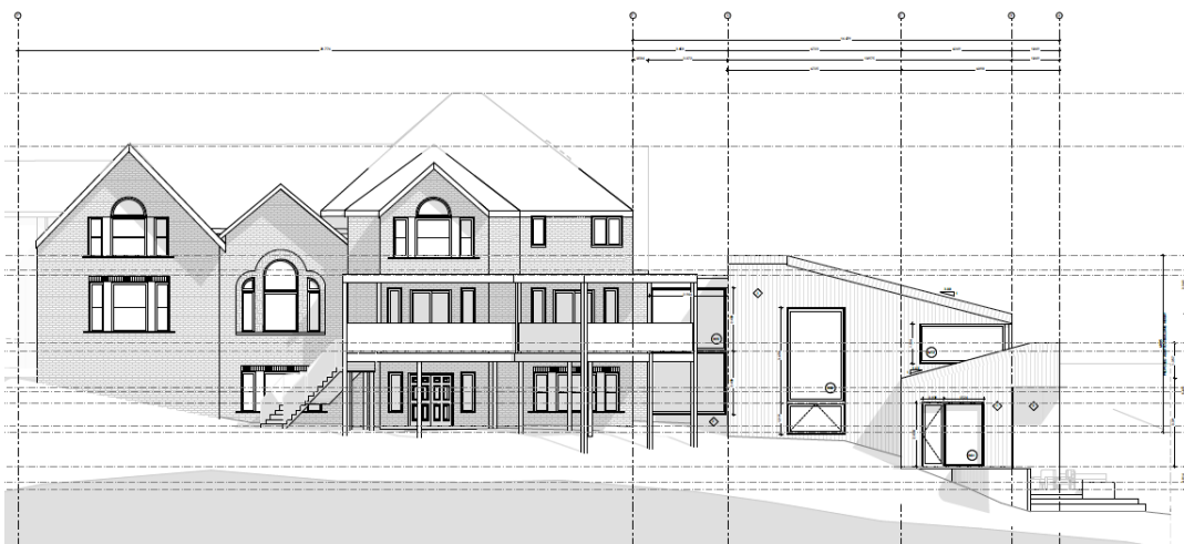
Rear Elevation
