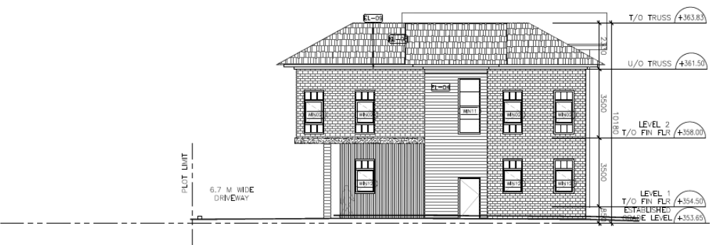
Side (Southeast) Elevation
