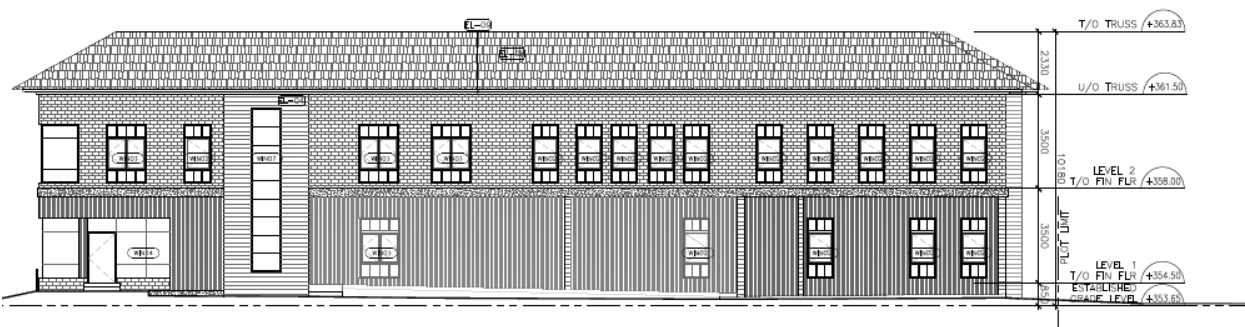
Side (Northwest) Elevation along York Street
